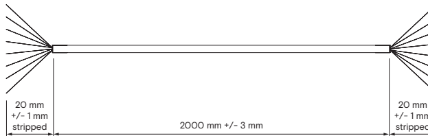
Cable - 2m ø4.0 straight (1001012)
